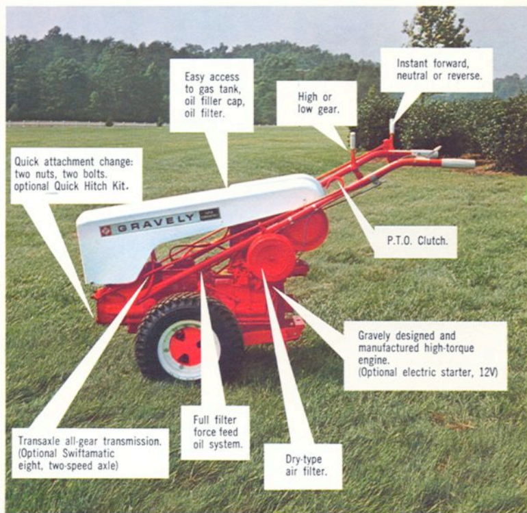
7.6 HP TRACTOR
