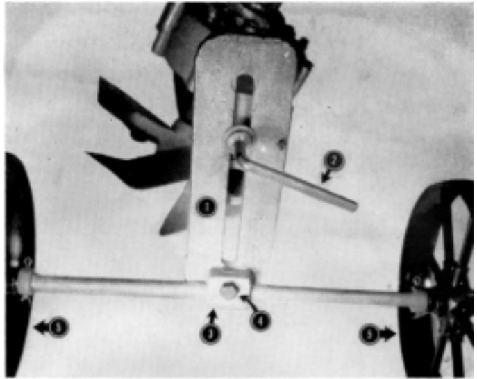
PLATE 35 (1) Wheel Bracket, (2) Wheel Bracket Clamp, (3) Axle Clamp, (4) Axle Clamp Screw, (5) Depth Wheel.
