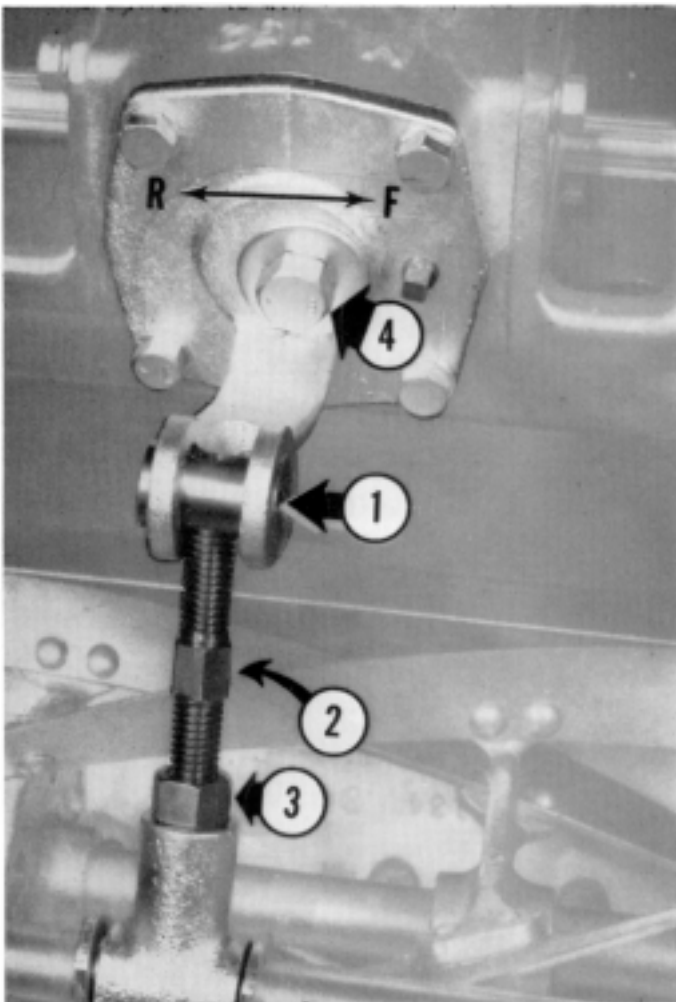
PLATE 16 1. Adjusting Screw Nut 3. Adjusting Screw Lock Nut 2. Adjusting Screw 4. Shifting Fork Bolt (R position reverses, F position is forward)
