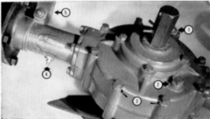
PLATE 34 (1) Depth Adjusting Clip, (2) Oil Filler Plug, (3) Attach Dirt Shield by these bolts, (4) Swivel Alemite Fitting, (5) Angle Adjusting Handle.
