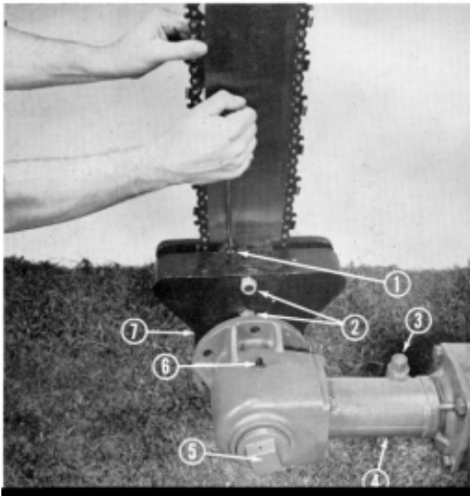
PLATE 25 (1) Chain Adjusting Screw, (2) Guide Bar Clamp Bolts, (3) Angle Adjustment Bolt, (4) Swivel Alemite Fitting, (5) Oil Filler Hole Plug, (6) Oil Level Hole Plug, (7) Bracket Clamp Nut.
