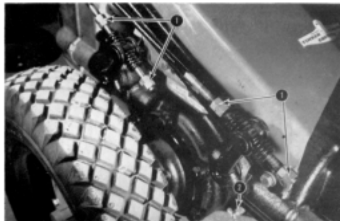
PLATE 2 (1) Clutch Adjusting Nuts, (2) Oil Level Try Cock.
