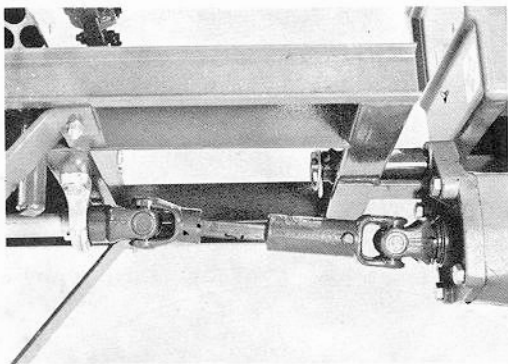
PTO shaft drive from tractor to shredder.
