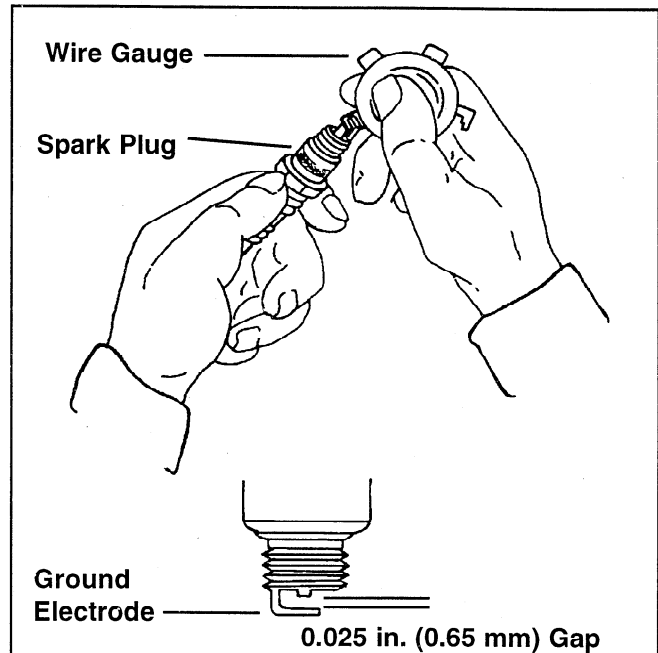
Figure 8. Servicing Spark Plug.
