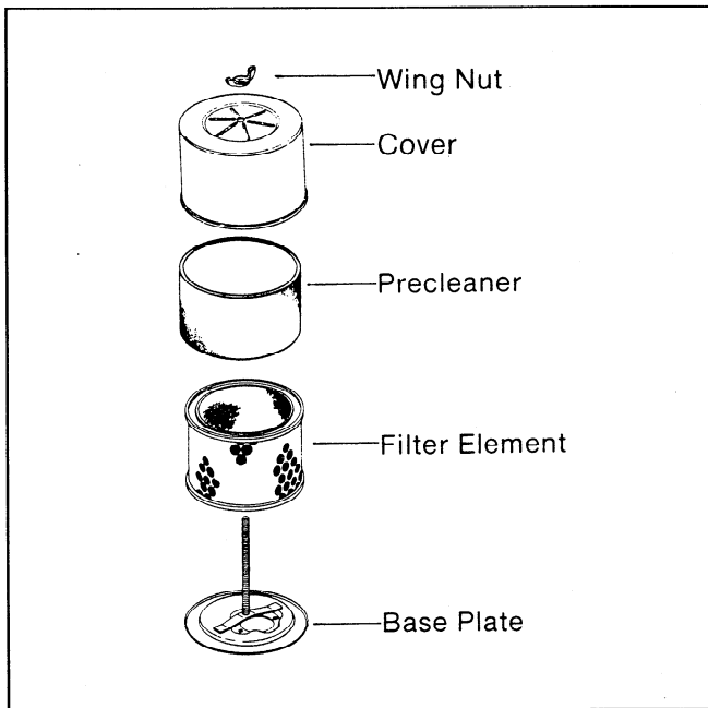
Figure 7. Air Cleaner Housing Components.
