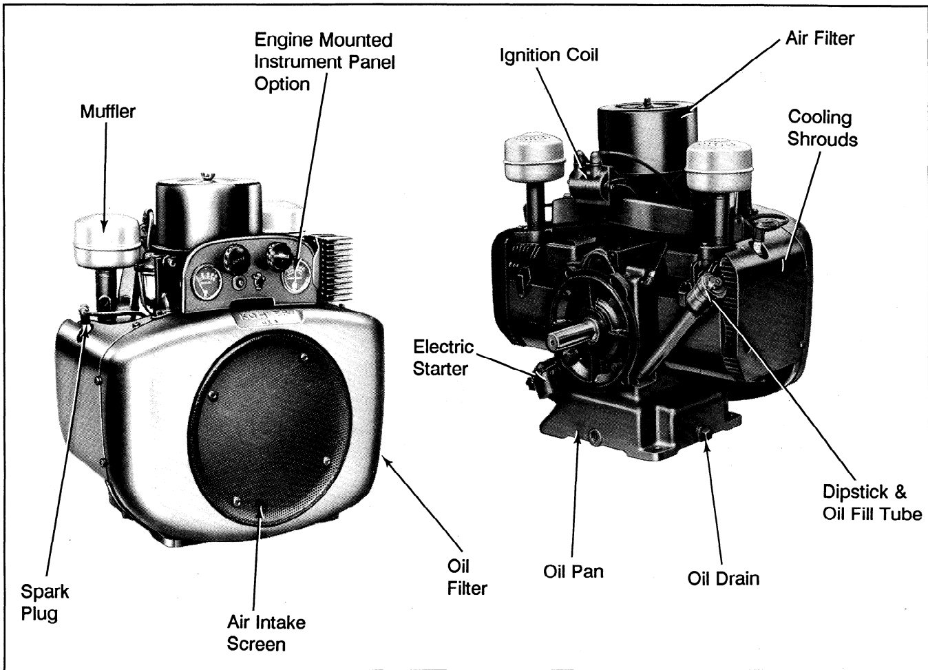
Figure 1. Typical K582 Engine.
