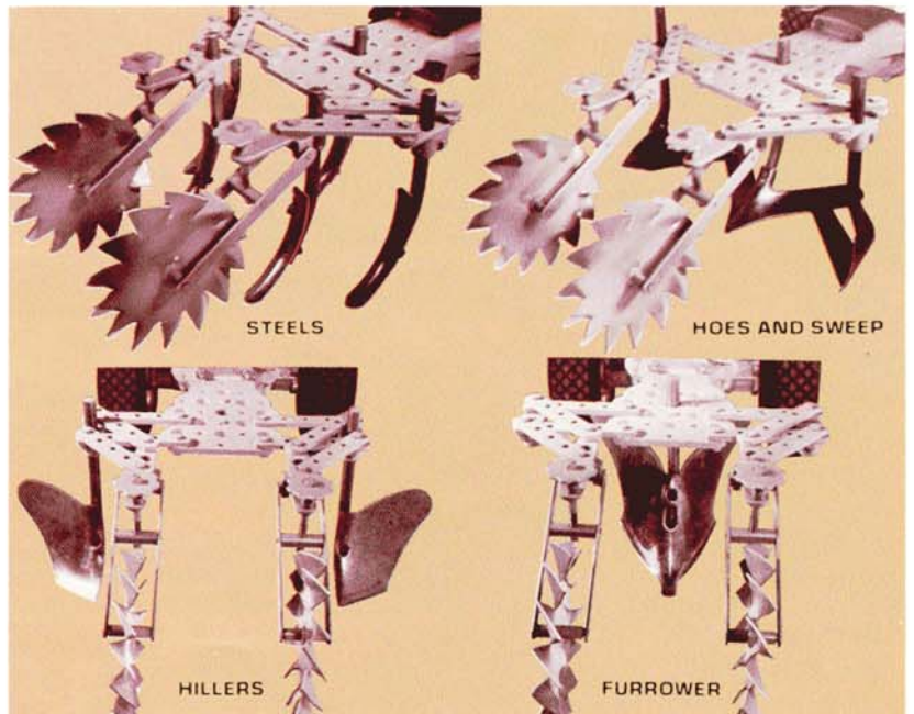
TOOL SET-UPS FOR TOOLHOLDERS
