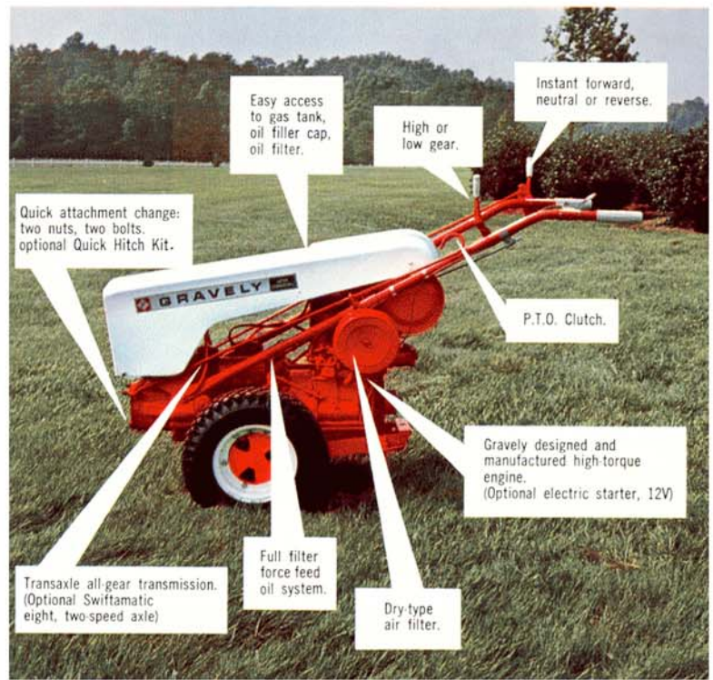
7.6 HP TRACTOR
