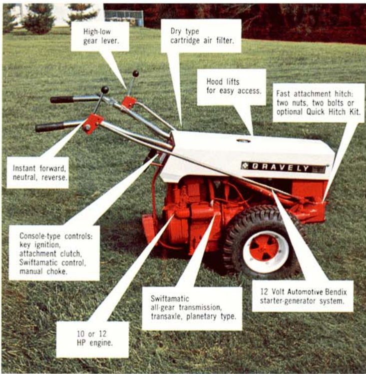
10 or 12 HP TRACTOR
